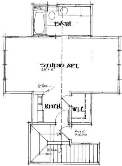
UPPER LEVEL FLOOR PLAN
