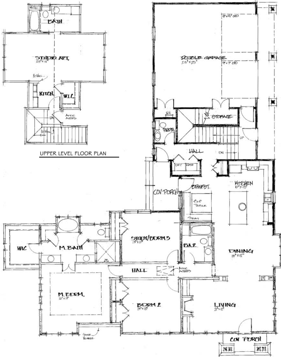
MAIN LEVEL FLOOR PLAN
